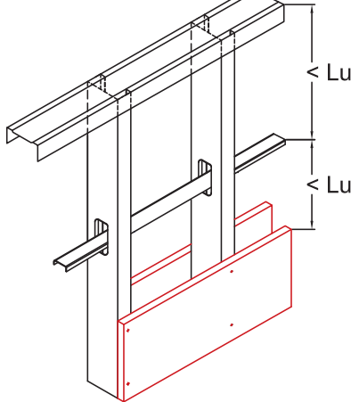
Non-Composite | Fully Braced Bracing spacing above gypsum is less than L_u
