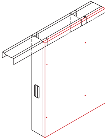
Non-Composite | Fully Braced Gypsum board full height
