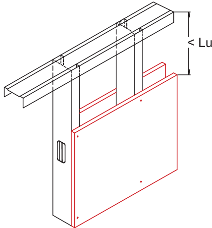
Non-Composite | Fully Braced Unbraced length is less than L_u
